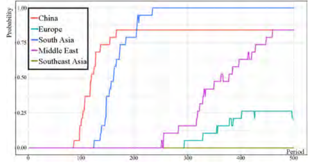
Figure 23: Probability of a large state arising in China, Europe, India, Middle East, or Southeast Asia (Incorporating the Steppe Effect).
