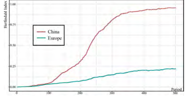
Figure 18: Median Plot for 19 simulations with rivers.
